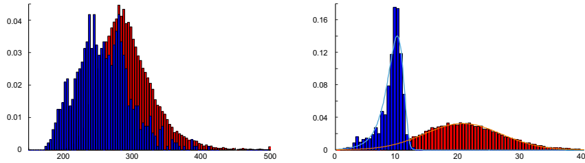
Fig. 4. Distribution of the scores o_t^{v,\alpha} before (left), and after training (right).
